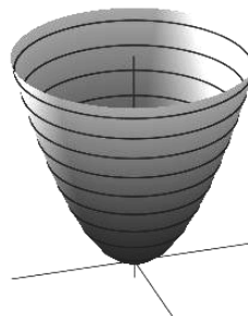
z = x^2 + y^2
